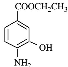
ethyl 4-amino-3-hydroxybenzoate
