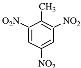
2,4,6-trinitrotoluene (TNT)
