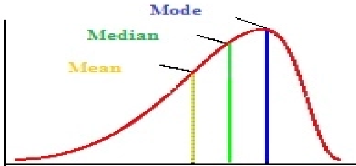
Left-Skewed (Negative Skewness)
