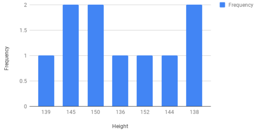
Frequency vs. Height
