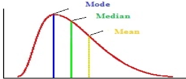
Right-Skewed (Positive Skewness)
